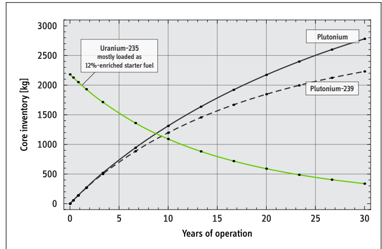
Figure 4.4: Build-up of plutonium in a 200-megawatt lifetime core-reactor (Family 4).
