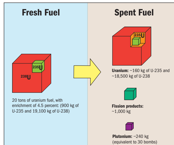
Figure 4.3: Annual flow of material through a 1,000-megawatt pressurized-water reactor. Figure adapted from http://www.laradioactivite.com/en/site/images/CompositionCUen.jpgimages/CompositionCUen.jpg
